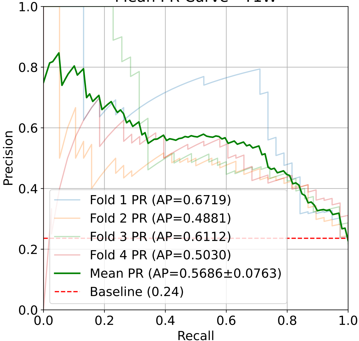
Mean PR Curve - T1W
